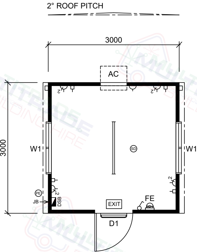
3.0x3.0m Open Plan Building - Floor Plan
